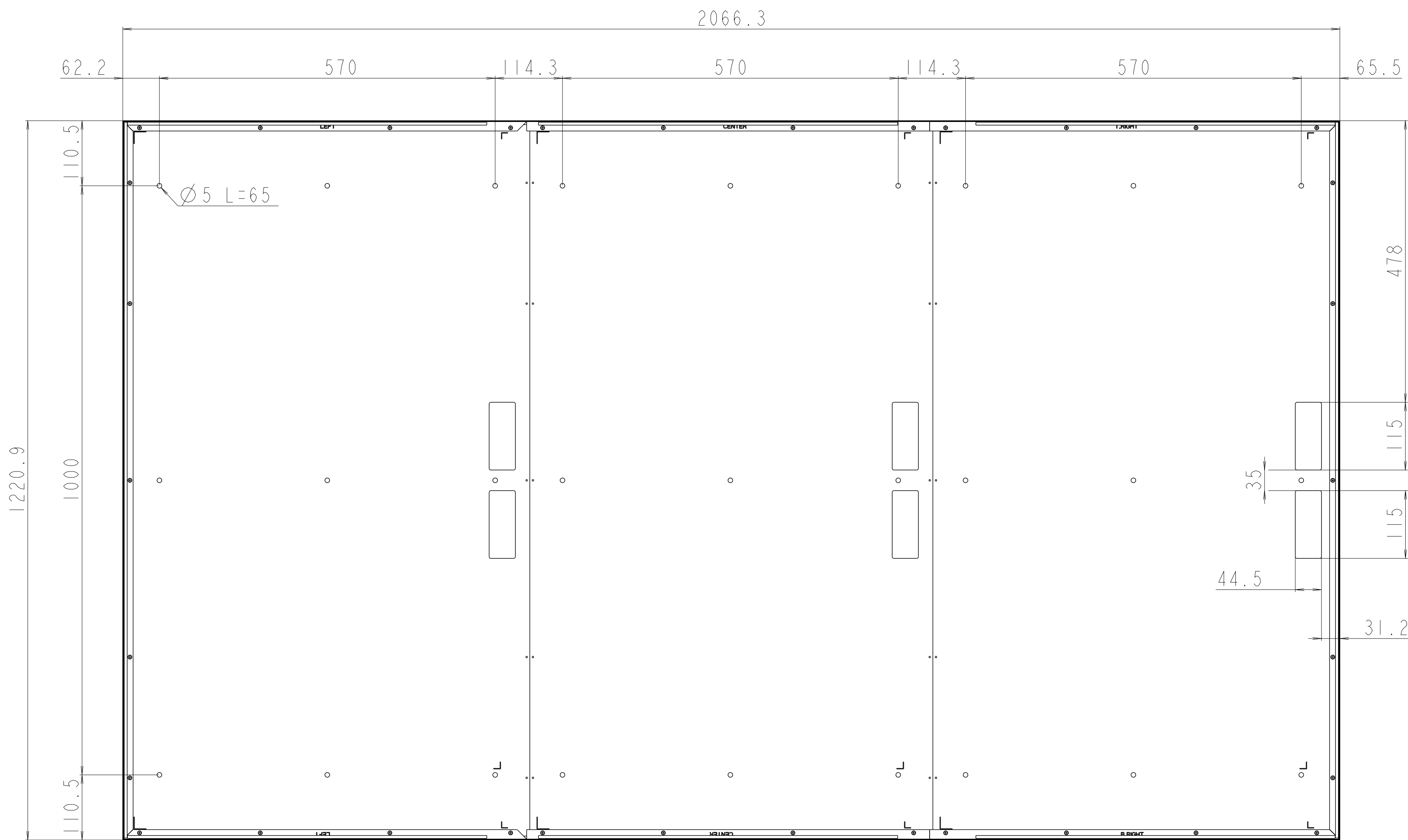
Anchor bolt position
