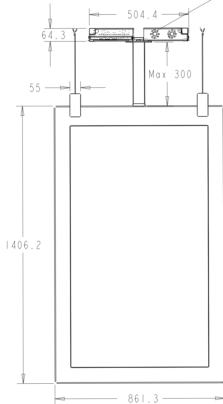
[Front View]
